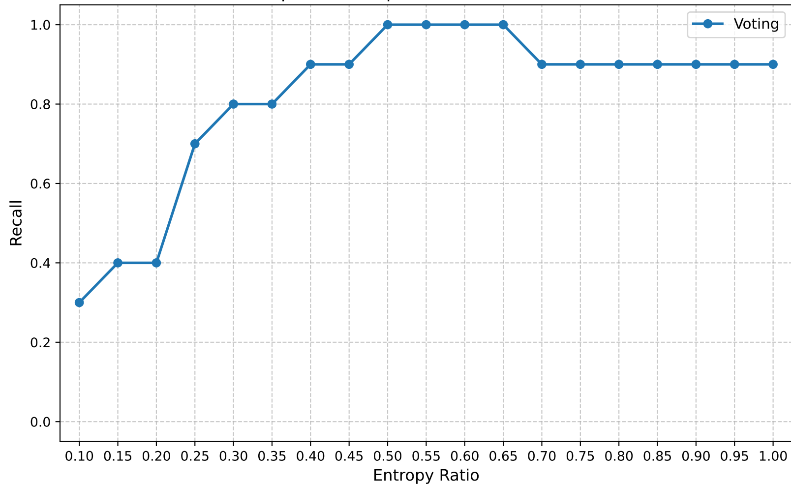
Recall | Round 15 | Confuse Model Ratio 0.70
