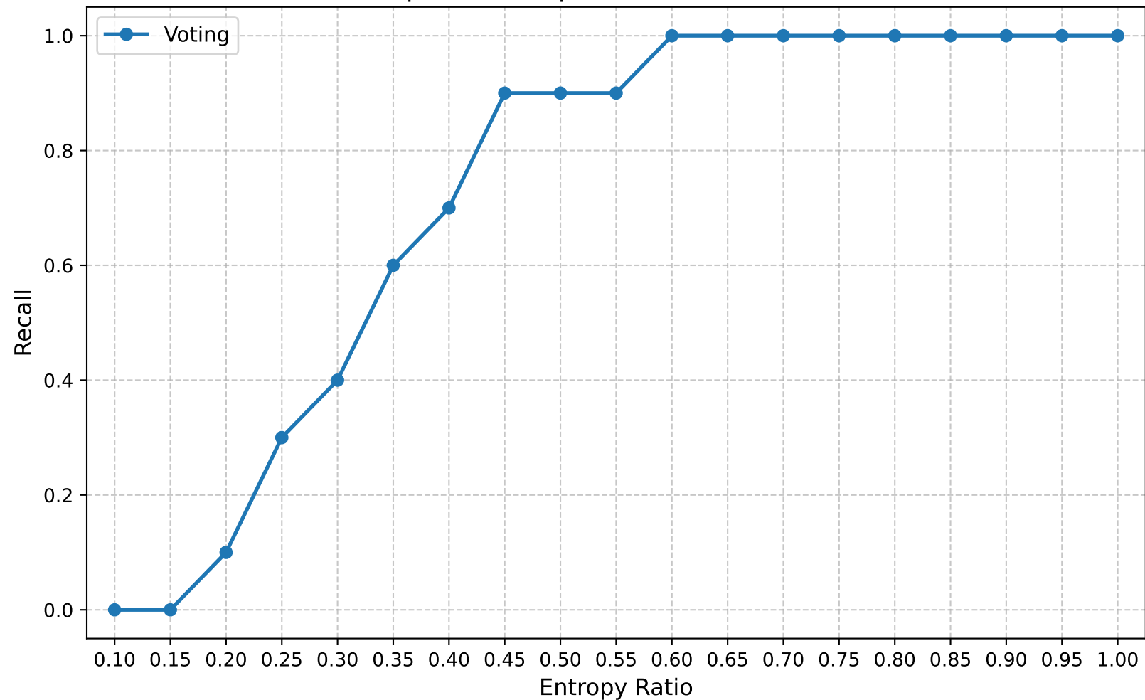
Recall | Round 20 | Confuse Model Ratio 0.40
