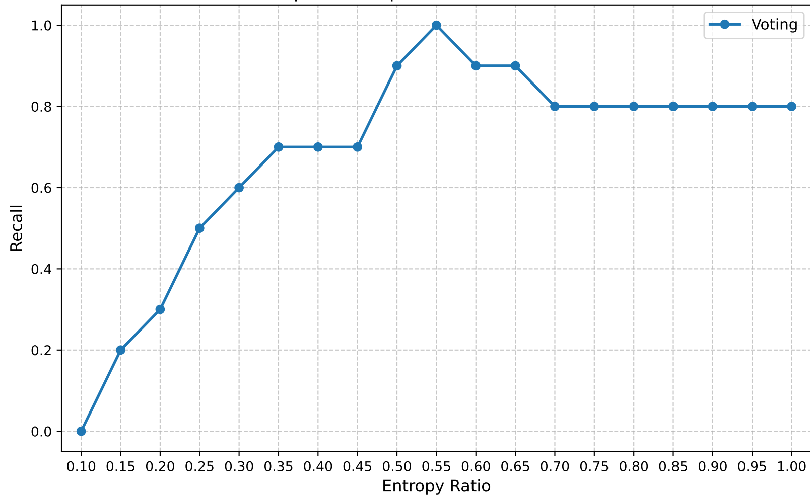
Recall | Round 5 | Confuse Model Ratio 0.40
