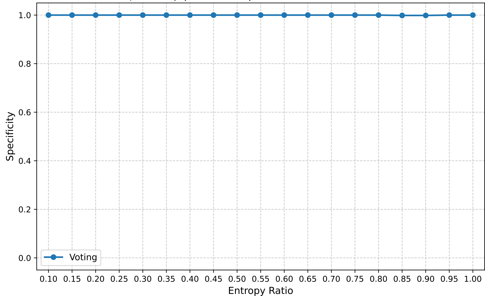
Specificity | Round 15 | Confuse Model Ratio 0.50
