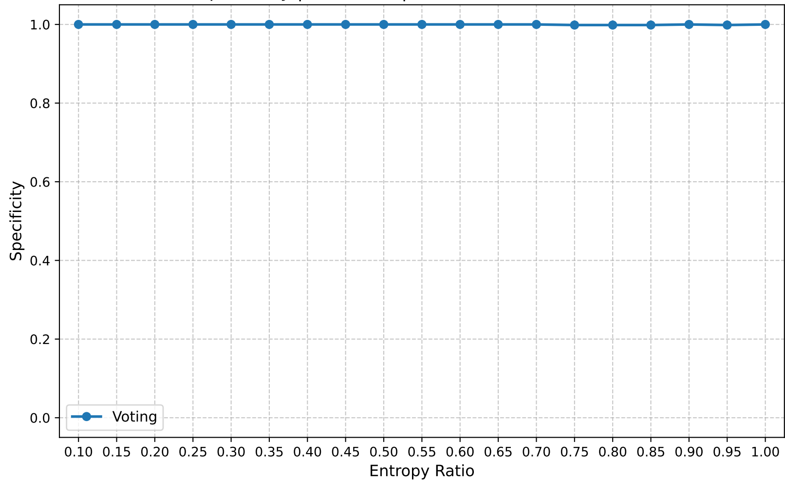
Specificity | Round 20 | Confuse Model Ratio 0.60
