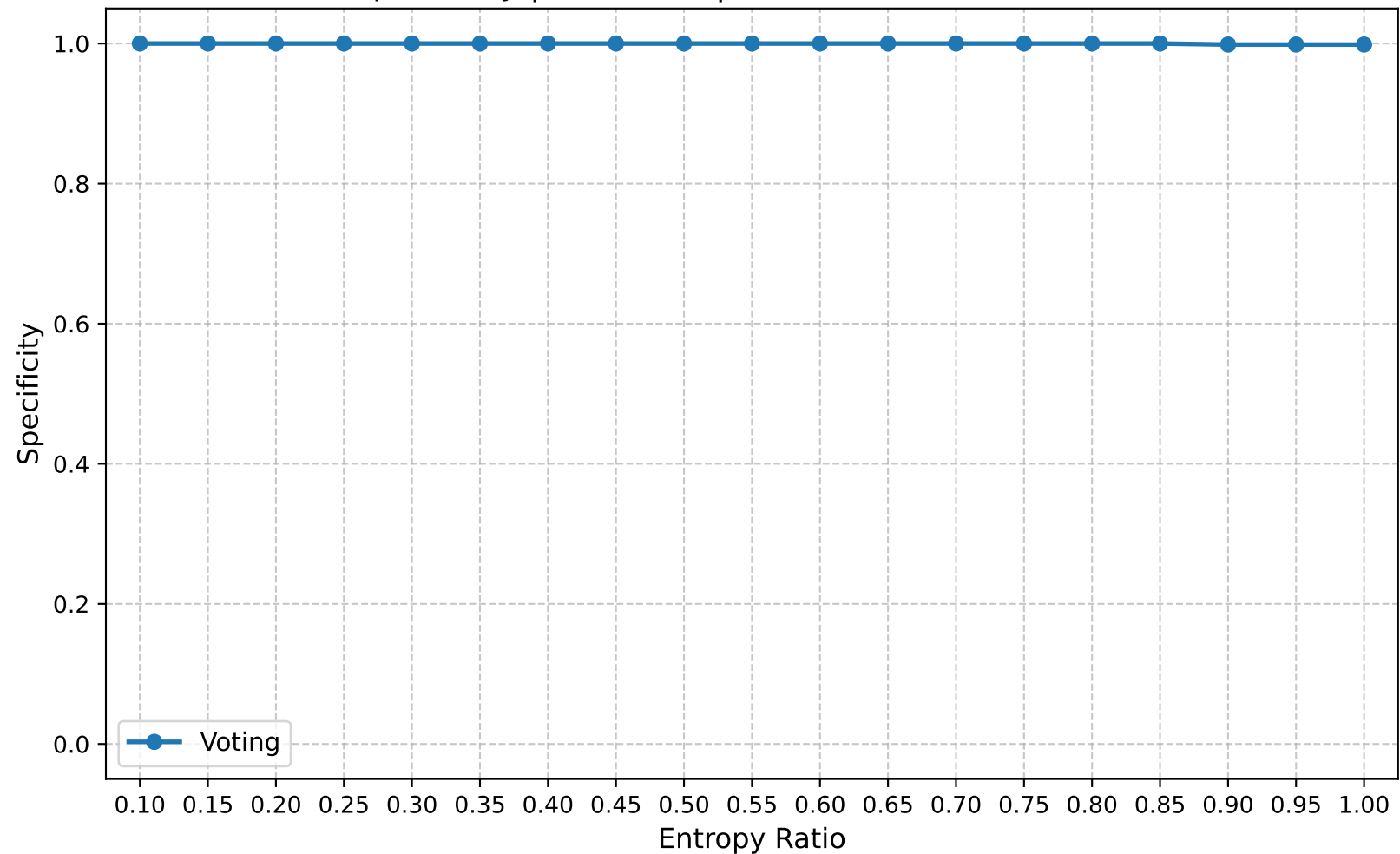
Specificity | Round 25 | Confuse Model Ratio 0.40
