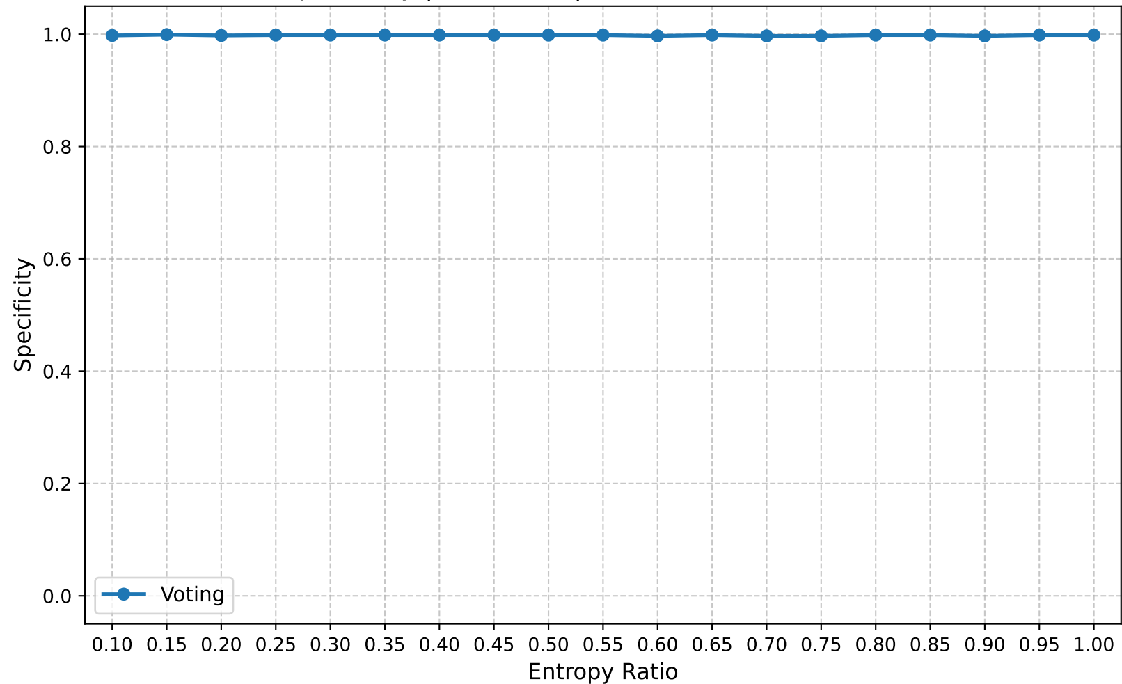
Specificity | Round 25 | Confuse Model Ratio 0.90
