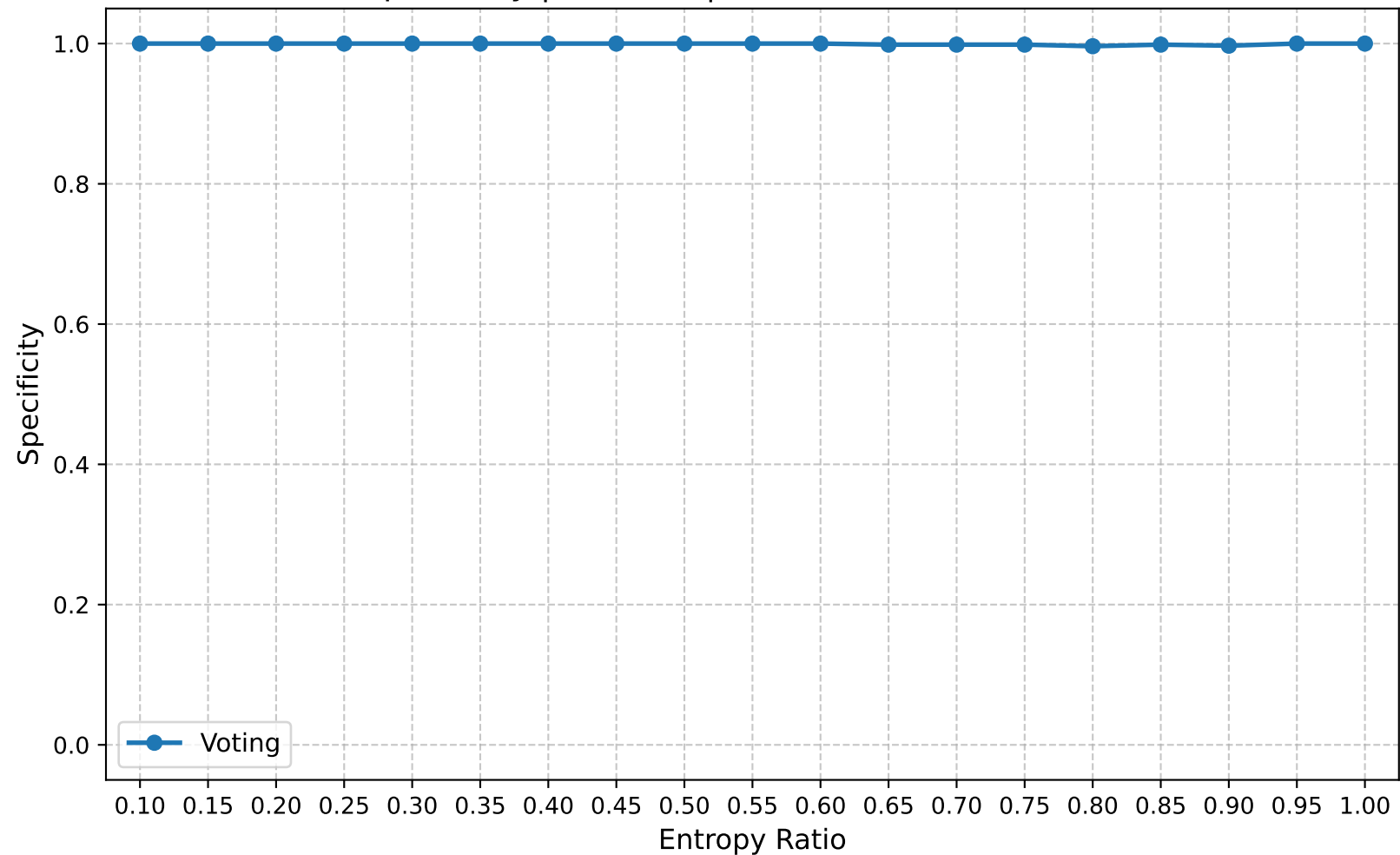
Specificity | Round 5 | Confuse Model Ratio 0.70
