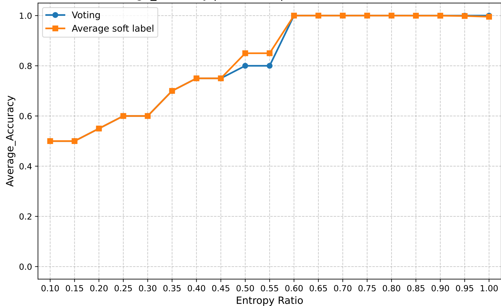
Average_Accuracy | Round 10 | Confuse Model Ratio 0.20
