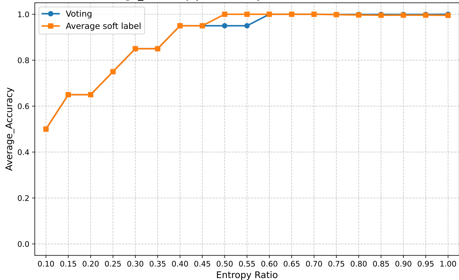
Average_Accuracy | Round 10 | Confuse Model Ratio 0.60
