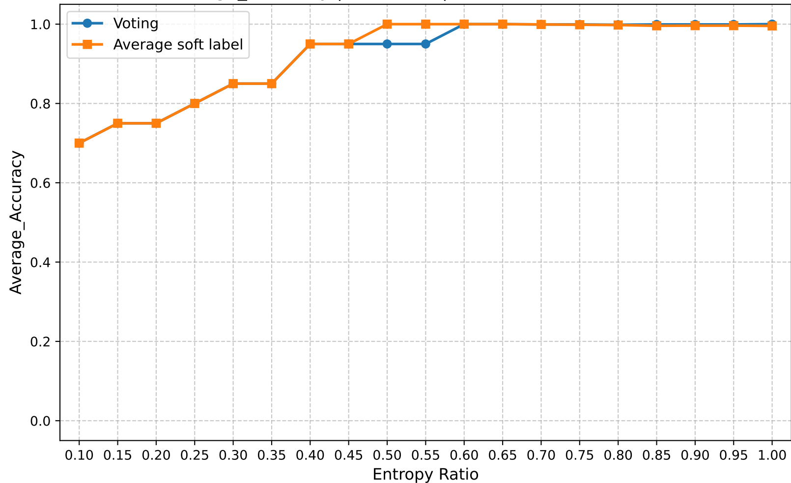
Average_Accuracy | Round 10 | Confuse Model Ratio 0.70
