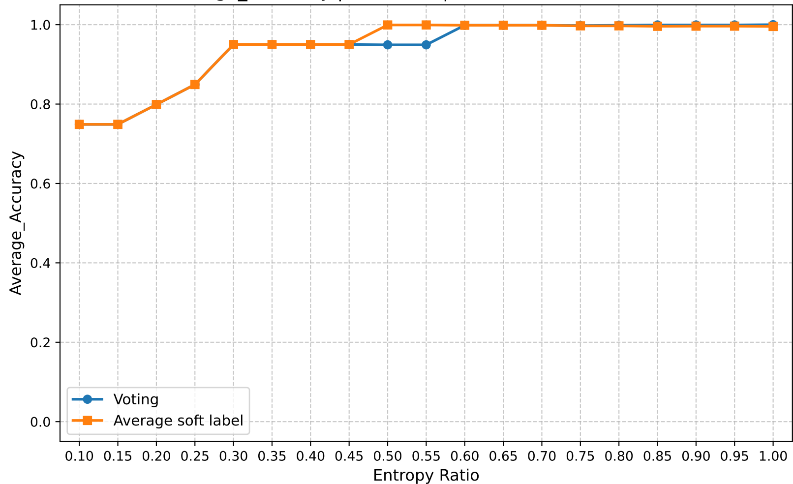
Average_Accuracy | Round 10 | Confuse Model Ratio 0.90
