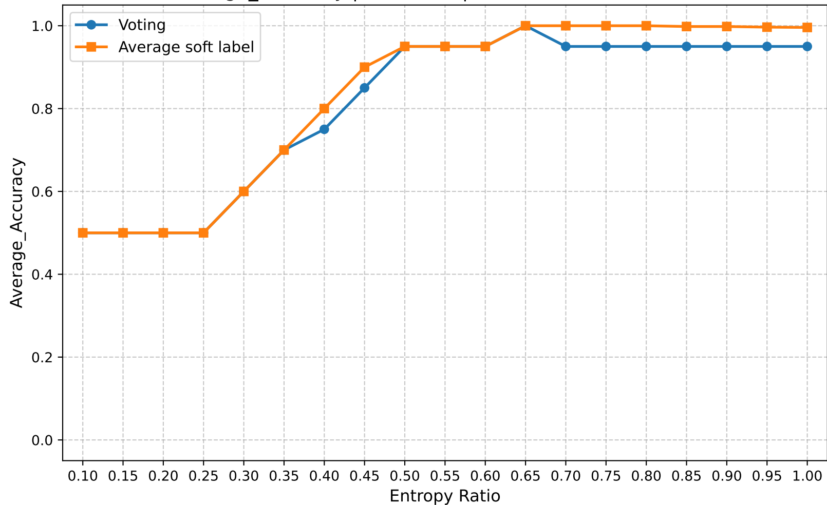
Average_Accuracy | Round 15 | Confuse Model Ratio 0.30
