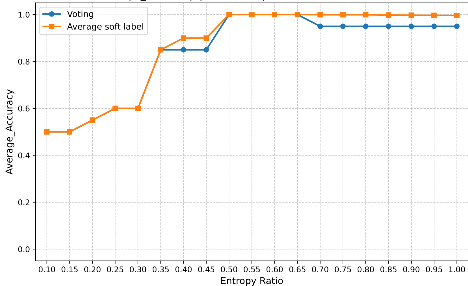
Average_Accuracy | Round 15 | Confuse Model Ratio 0.40
