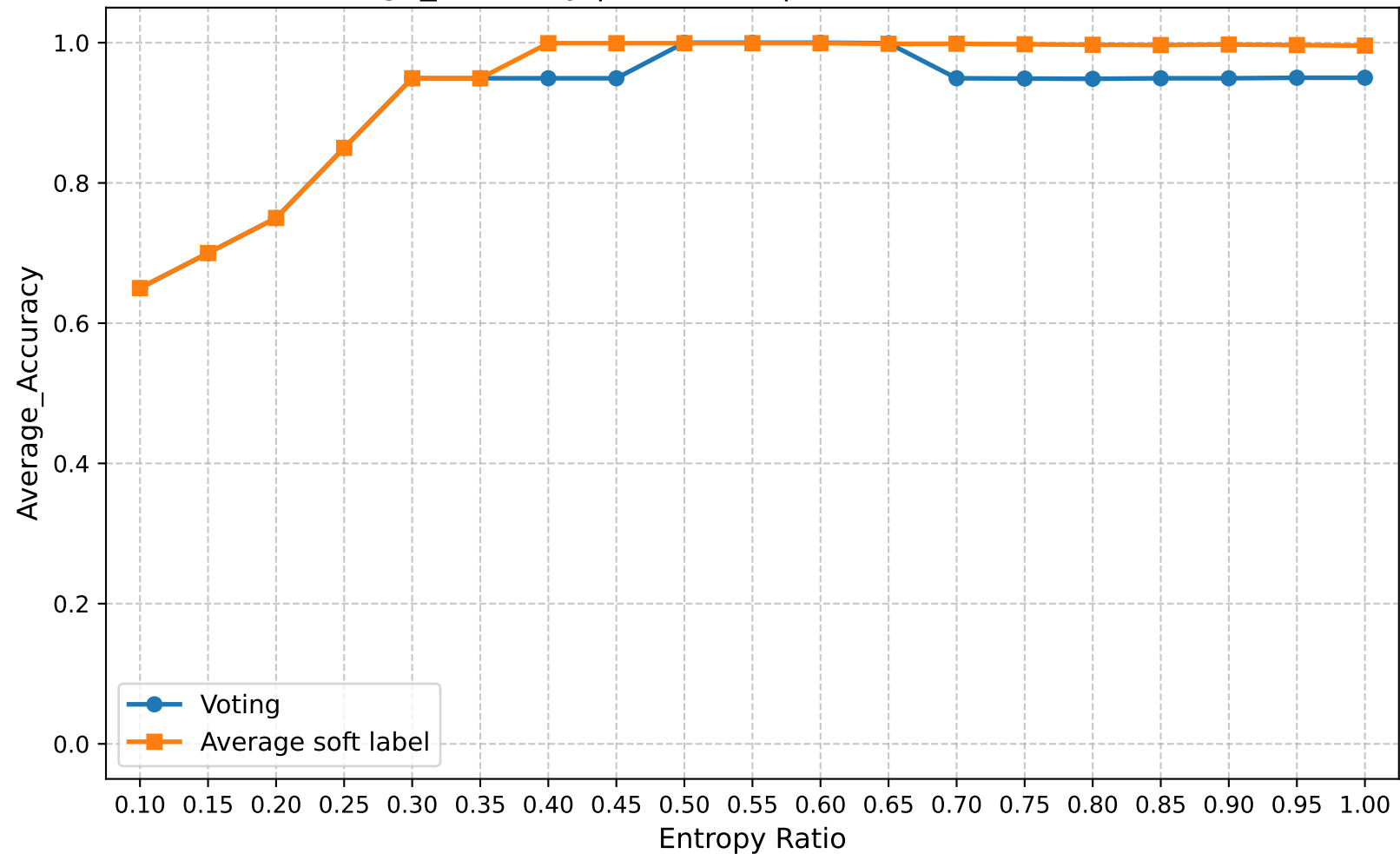
Average_Accuracy | Round 15 | Confuse Model Ratio 0.80
