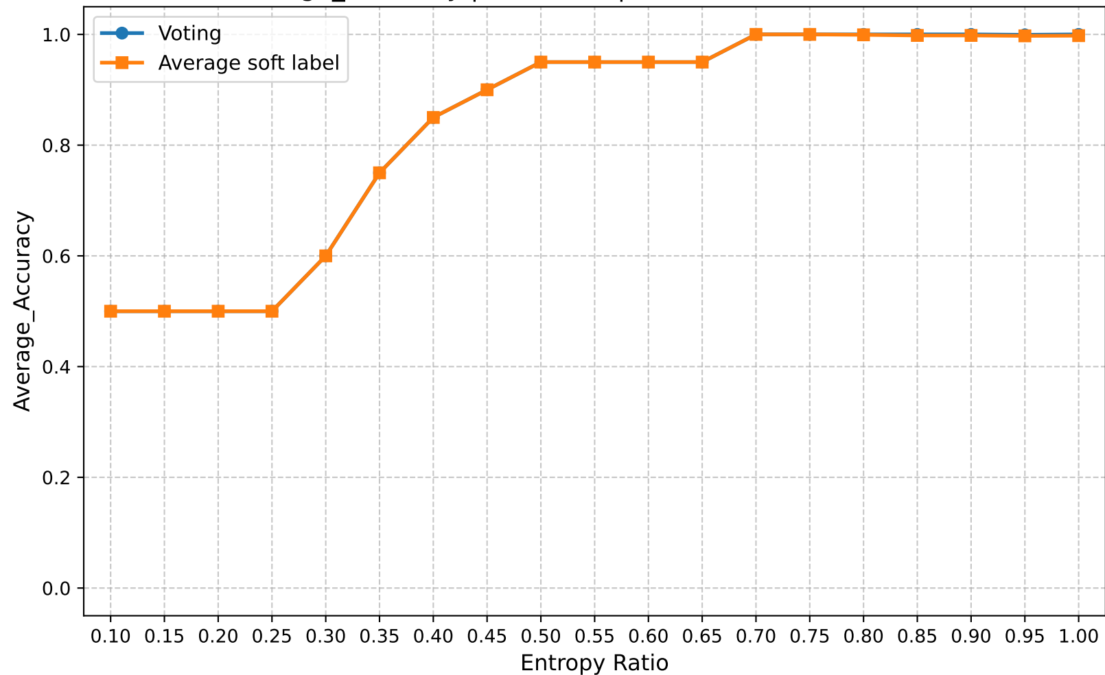
Average_Accuracy | Round 20 | Confuse Model Ratio 0.30
