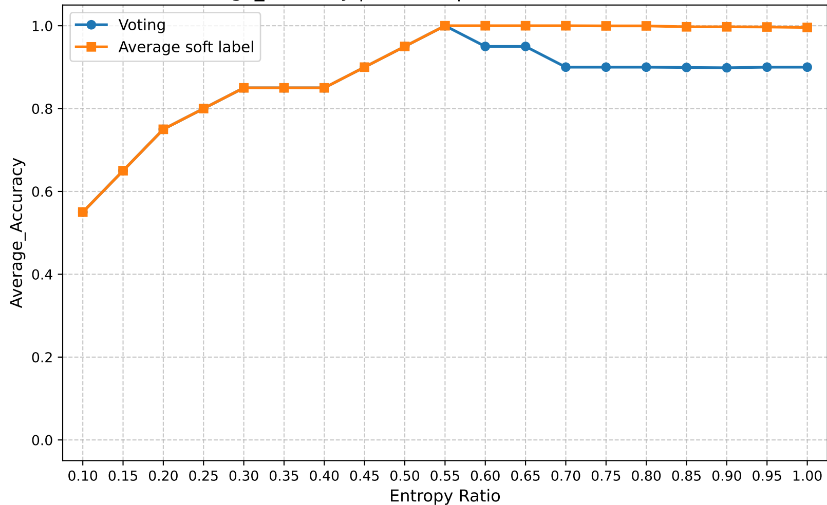
Average_Accuracy | Round 5 | Confuse Model Ratio 0.50
