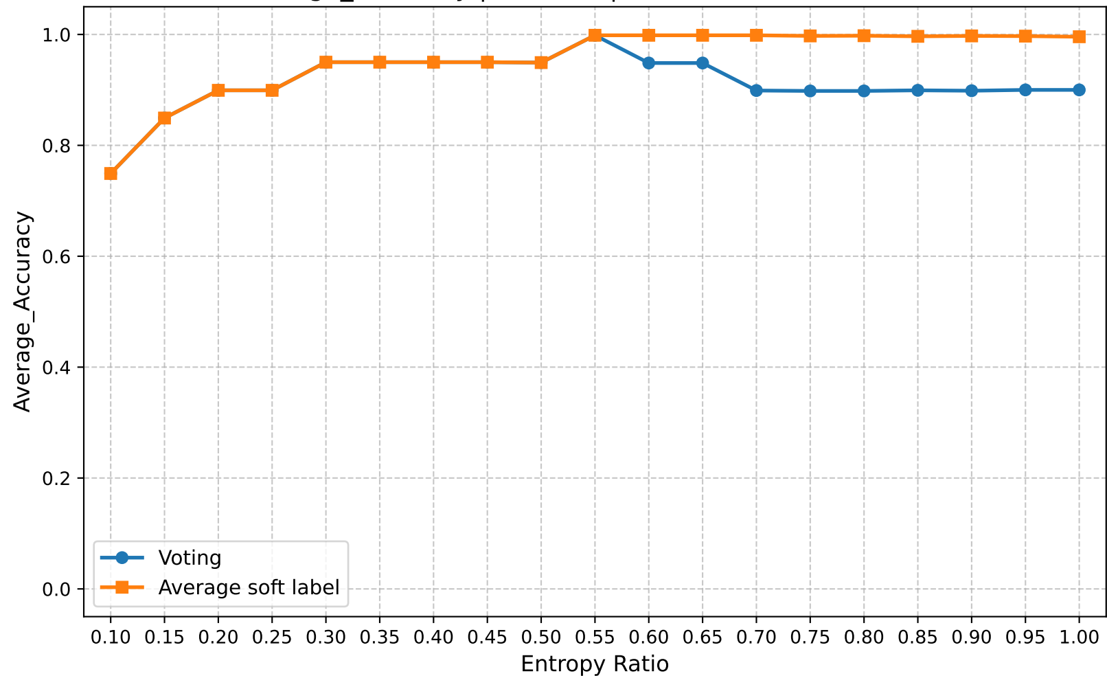
Average_Accuracy | Round 5 | Confuse Model Ratio 1.00
