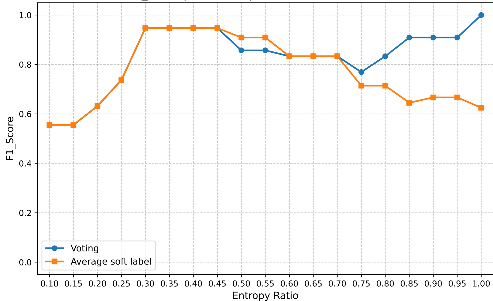
F1_Score | Round 10 | Confuse Model Ratio 1.00
