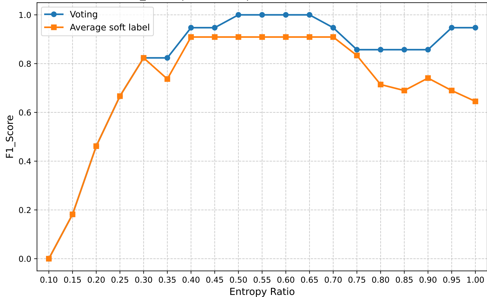
F1_Score | Round 15 | Confuse Model Ratio 0.60
