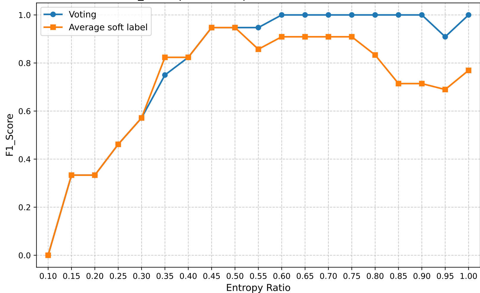
F1_Score | Round 20 | Confuse Model Ratio 0.50
