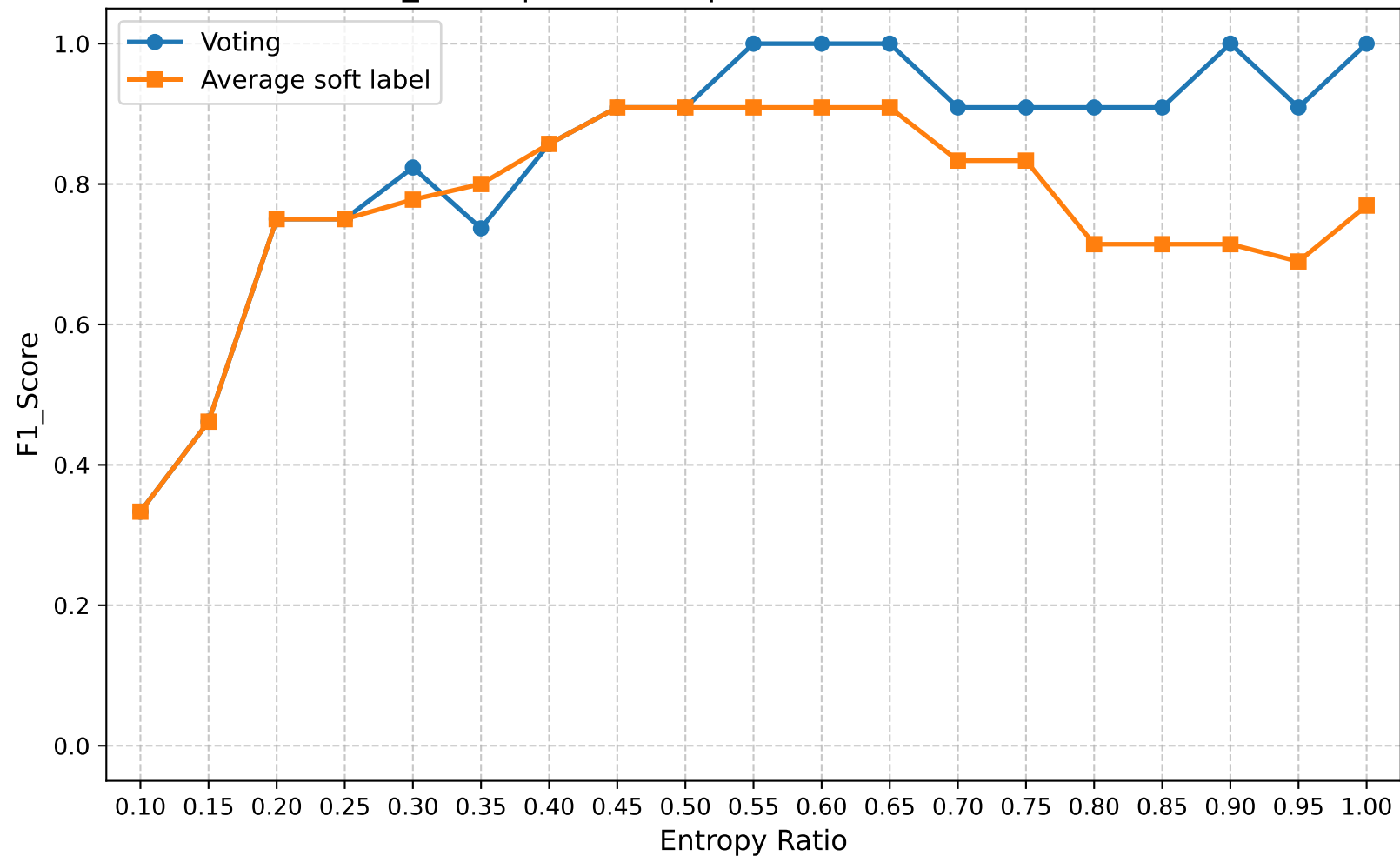
F1_Score | Round 20 | Confuse Model Ratio 0.70
