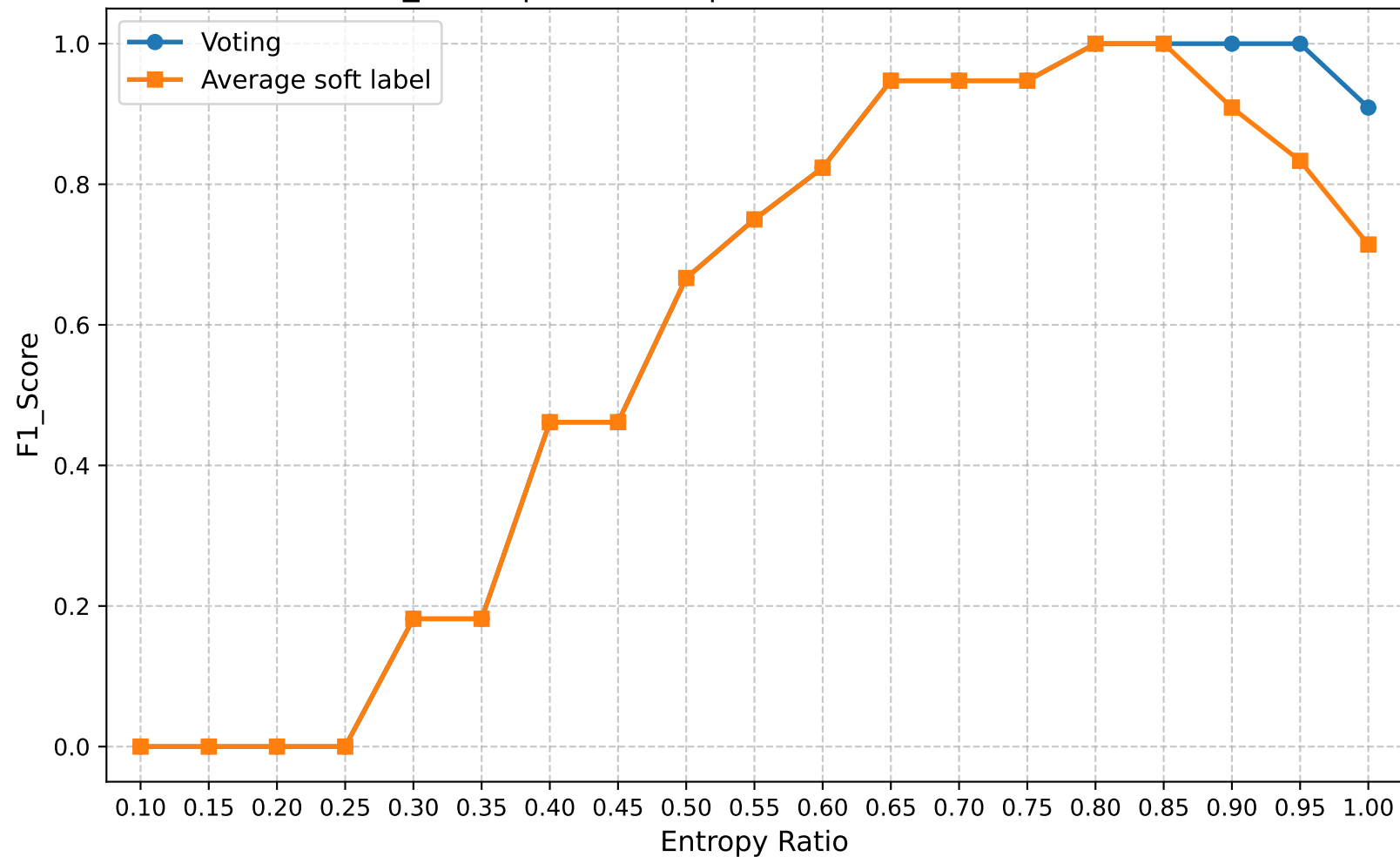
F1_Score | Round 25 | Confuse Model Ratio 0.10
