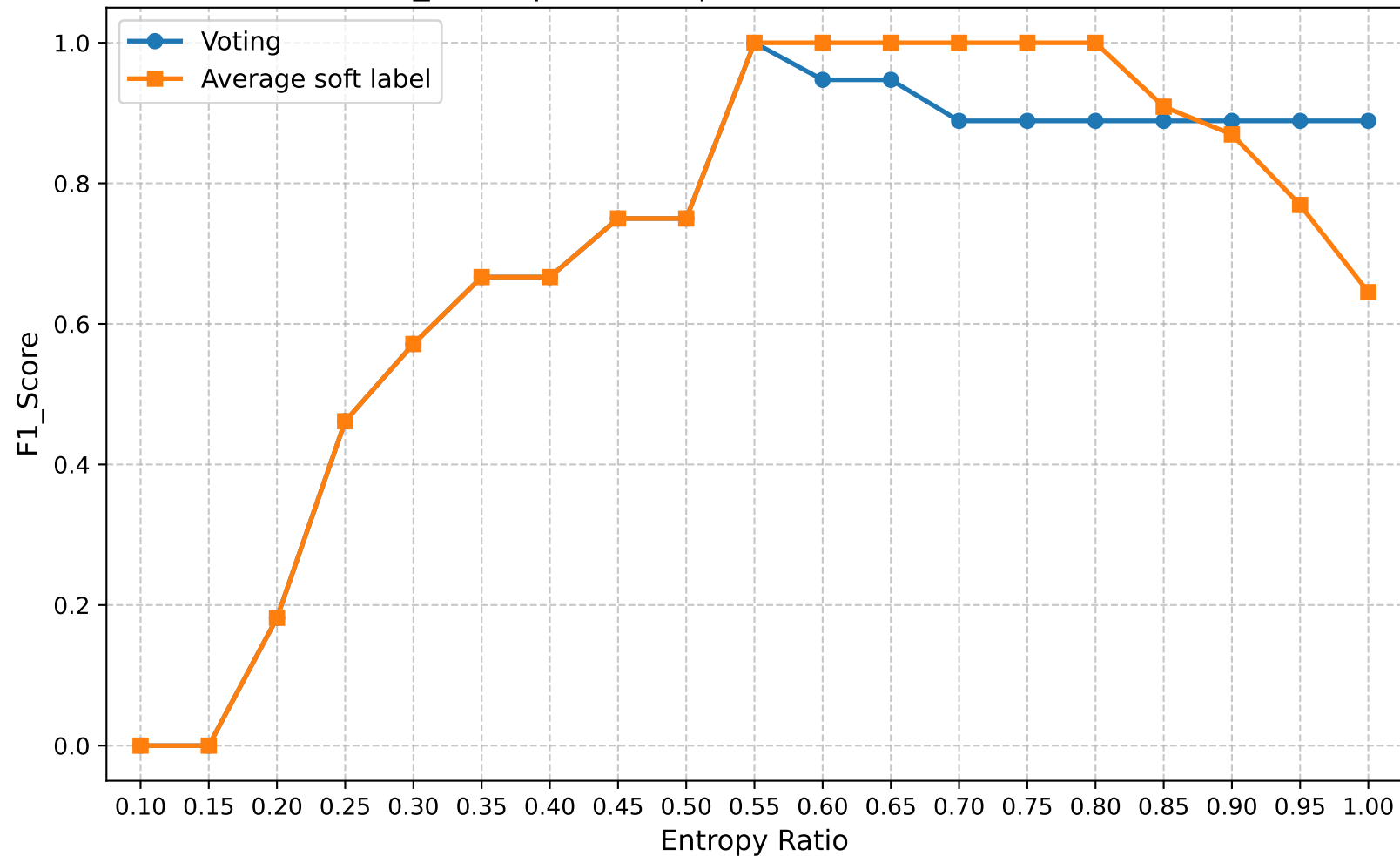
F1_Score | Round 5 | Confuse Model Ratio 0.20
