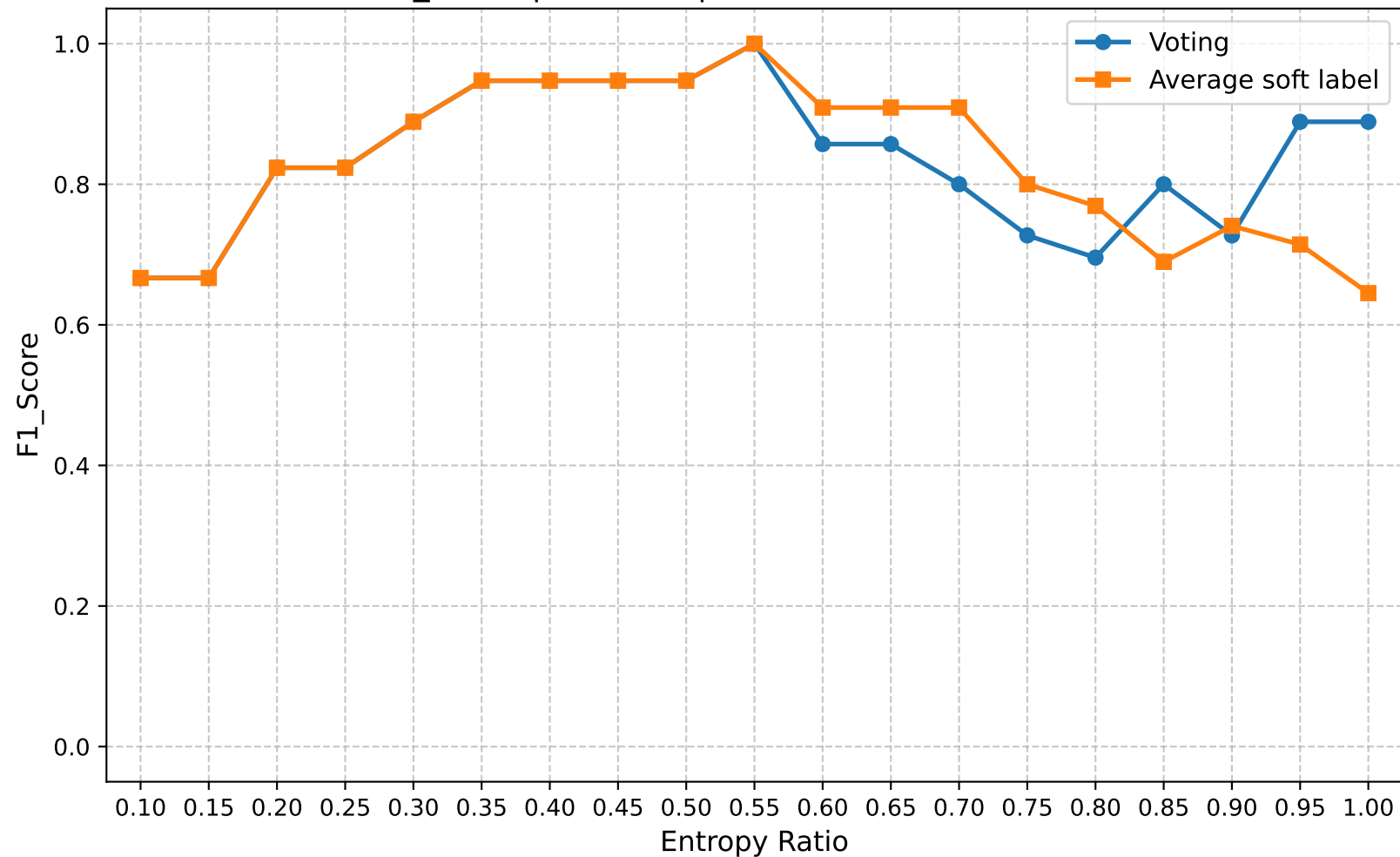
F1_Score | Round 5 | Confuse Model Ratio 0.80
