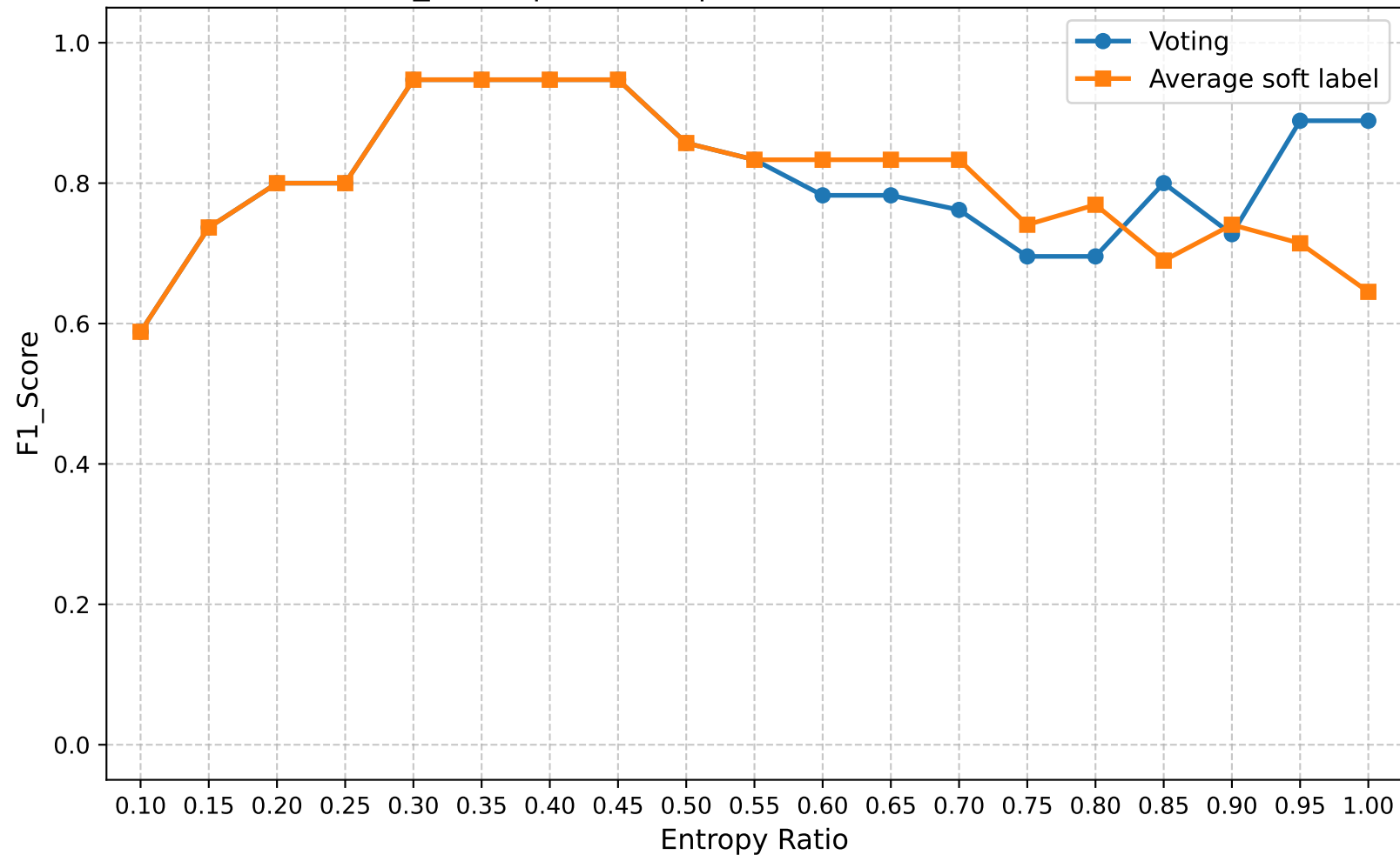
F1_Score | Round 5 | Confuse Model Ratio 0.90
