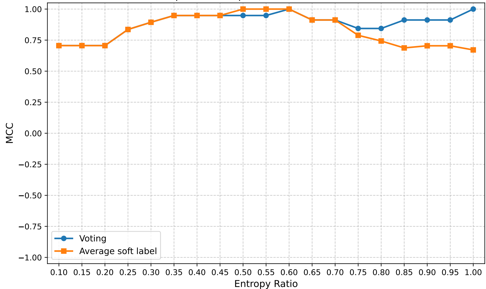
MCC | Round 10 | Confuse Model Ratio 0.80
