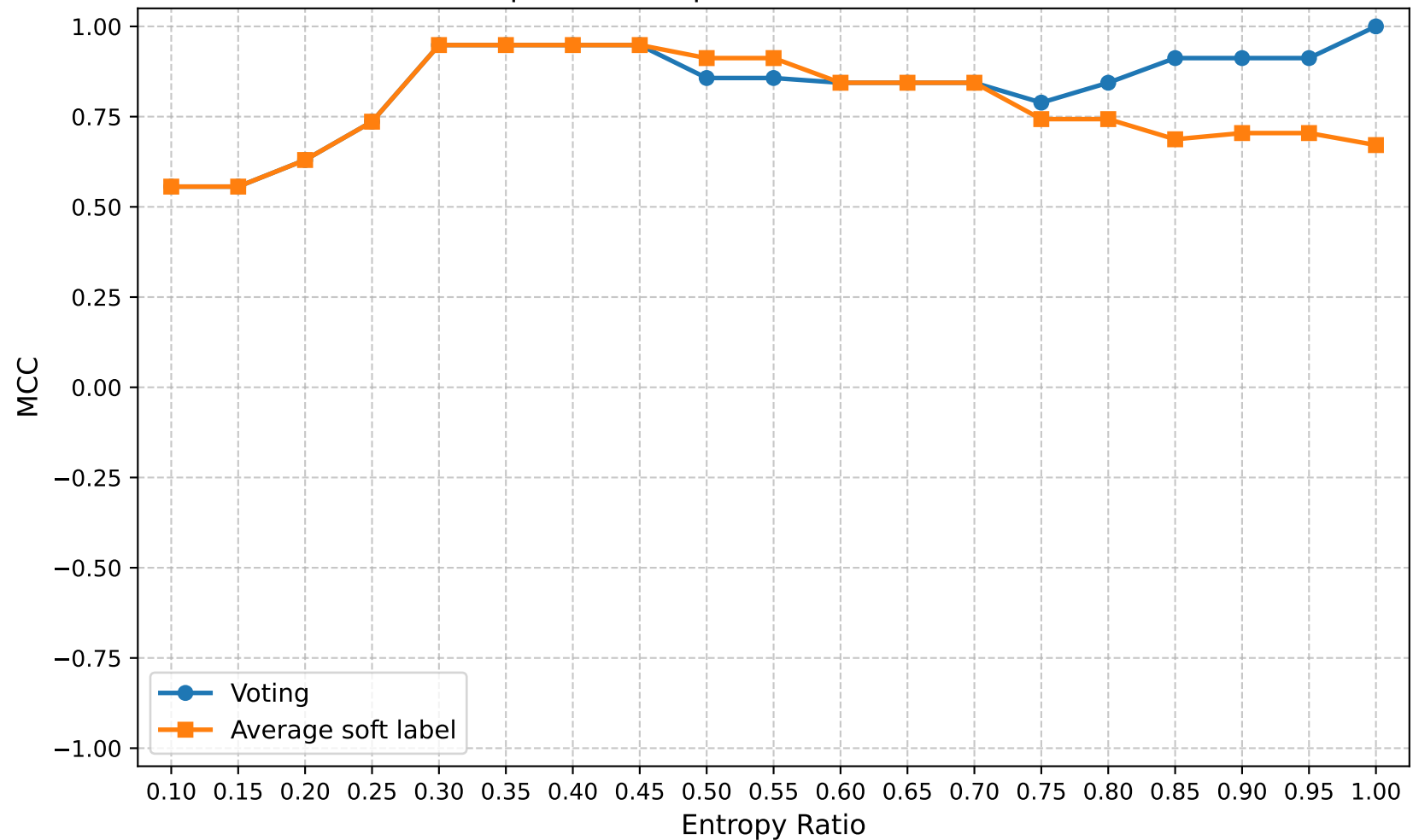
MCC | Round 10 | Confuse Model Ratio 0.90
