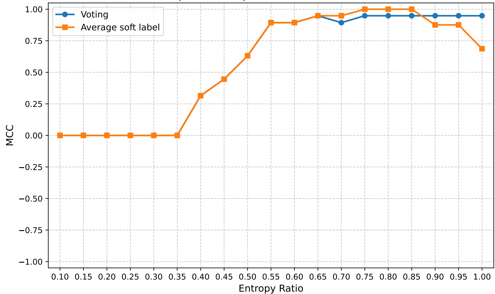
MCC | Round 15 | Confuse Model Ratio 0.10
