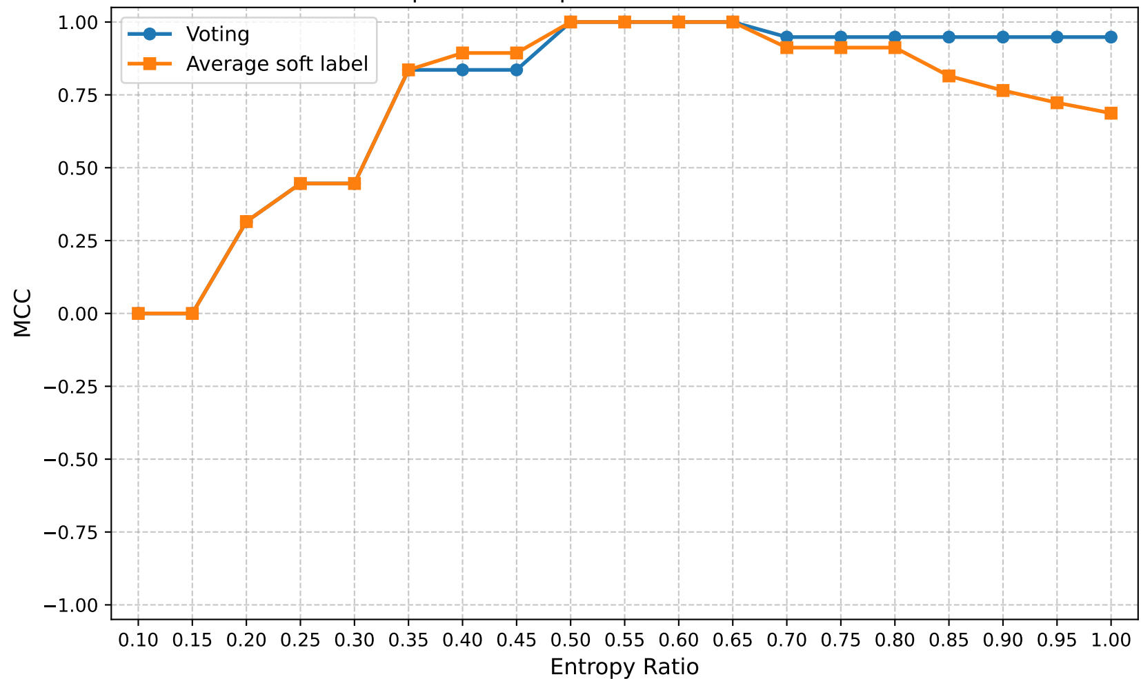
MCC | Round 15 | Confuse Model Ratio 0.40
