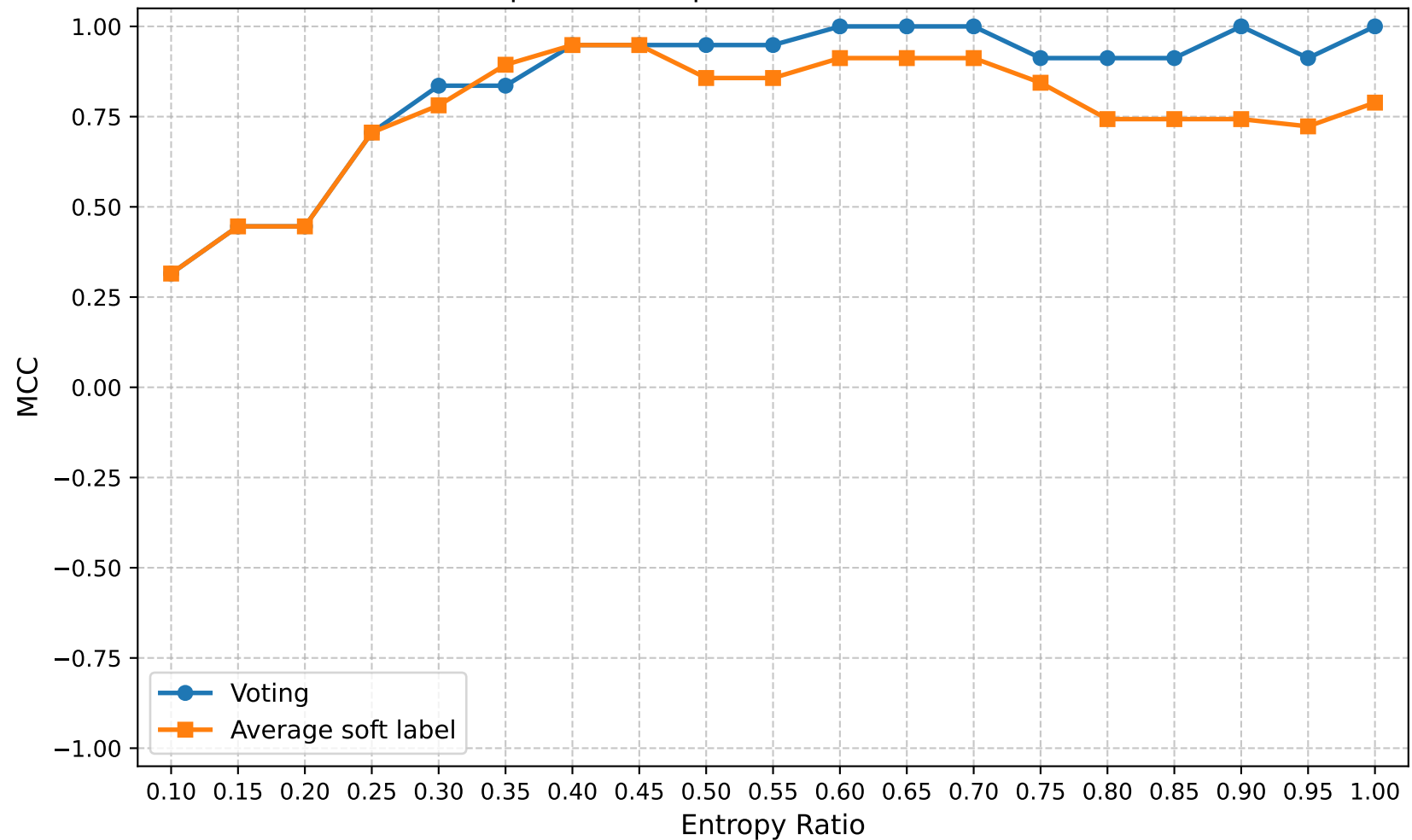
MCC | Round 20 | Confuse Model Ratio 0.60
