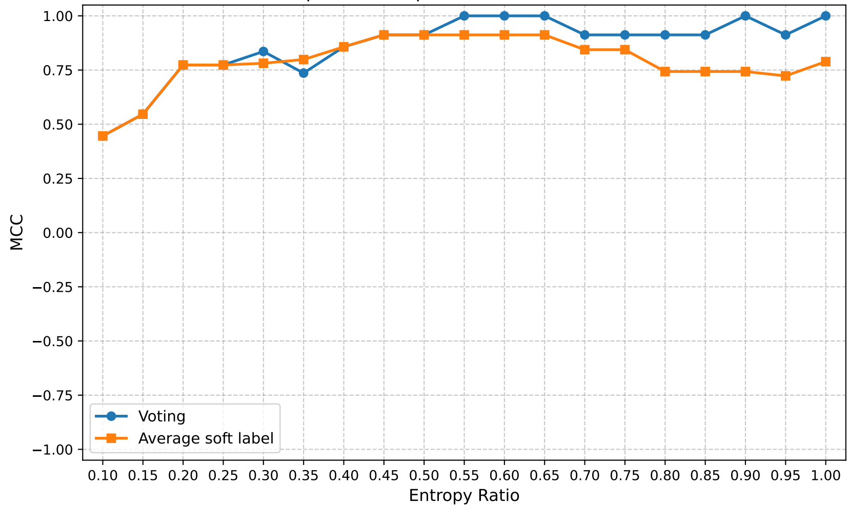
MCC | Round 20 | Confuse Model Ratio 0.70
