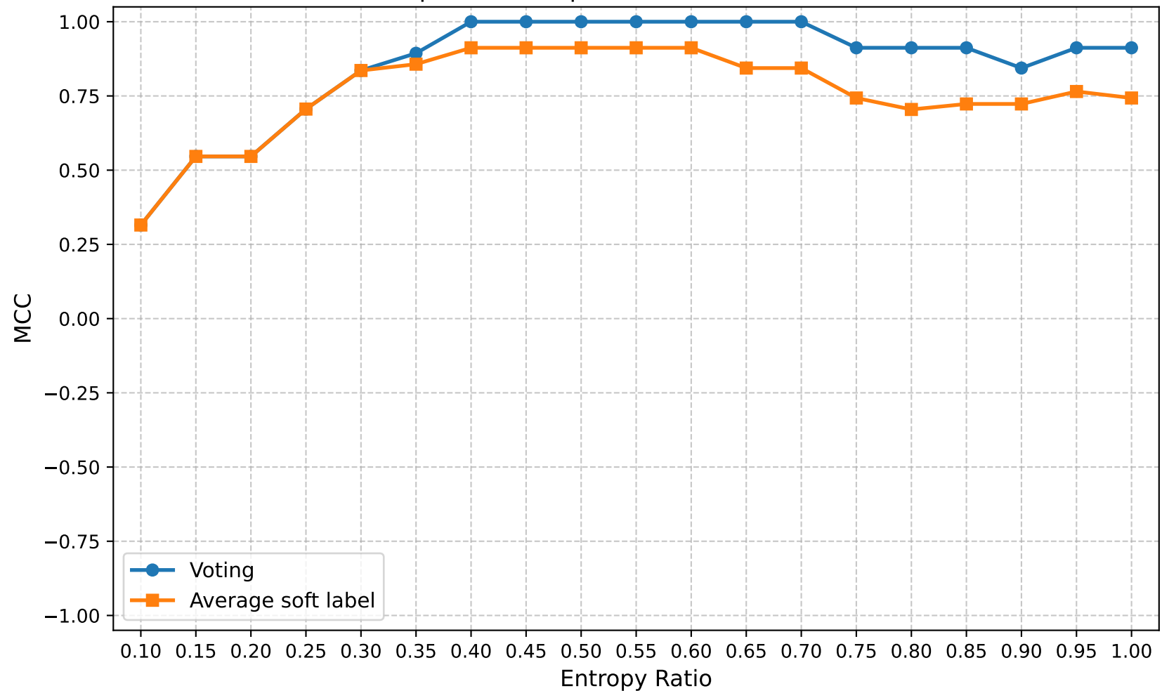
MCC | Round 25 | Confuse Model Ratio 0.60
