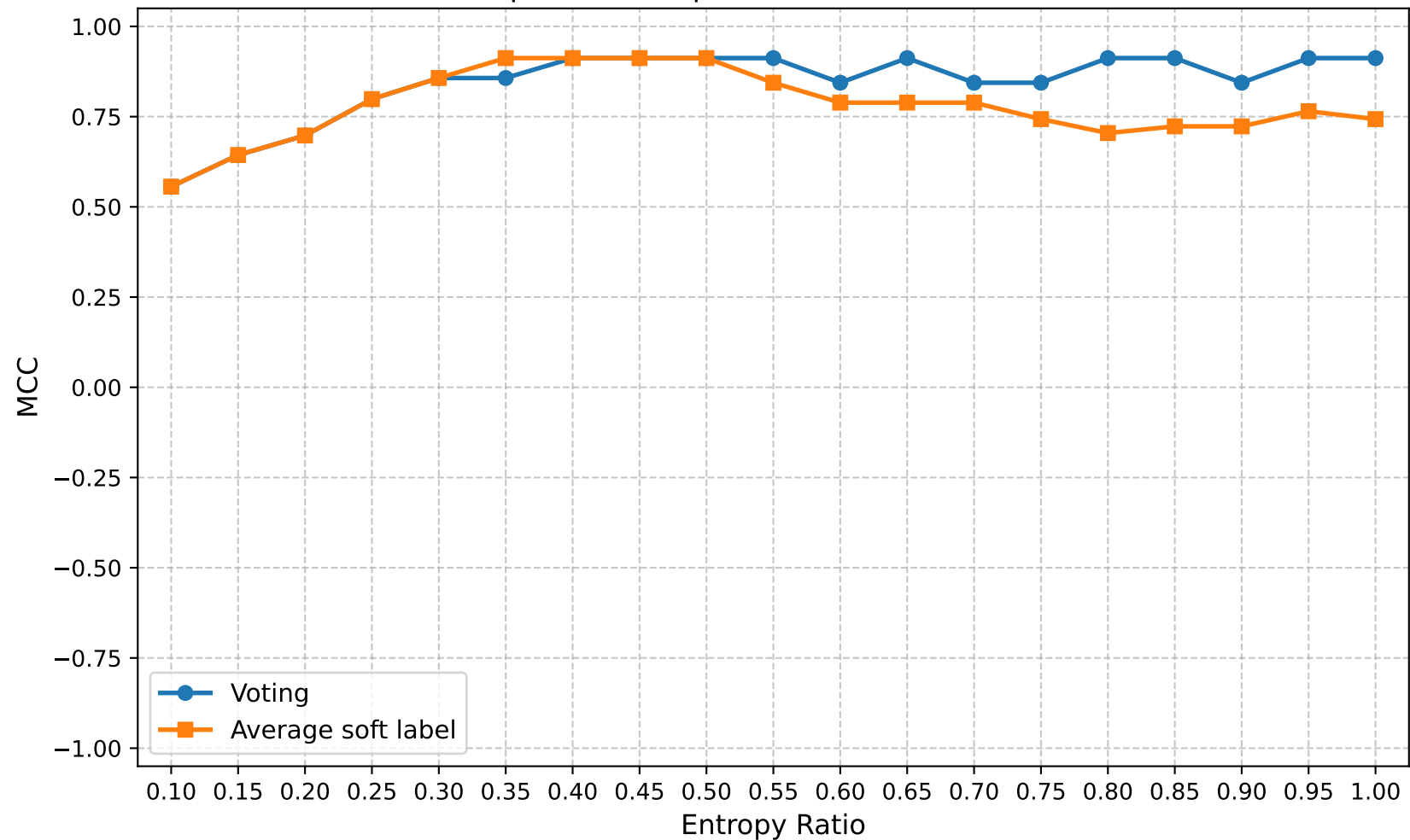
MCC | Round 25 | Confuse Model Ratio 0.90
