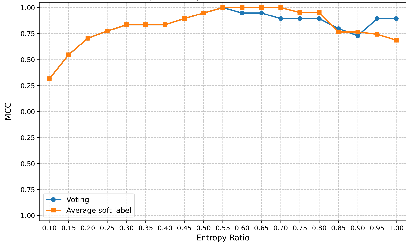
MCC | Round 5 | Confuse Model Ratio 0.50
