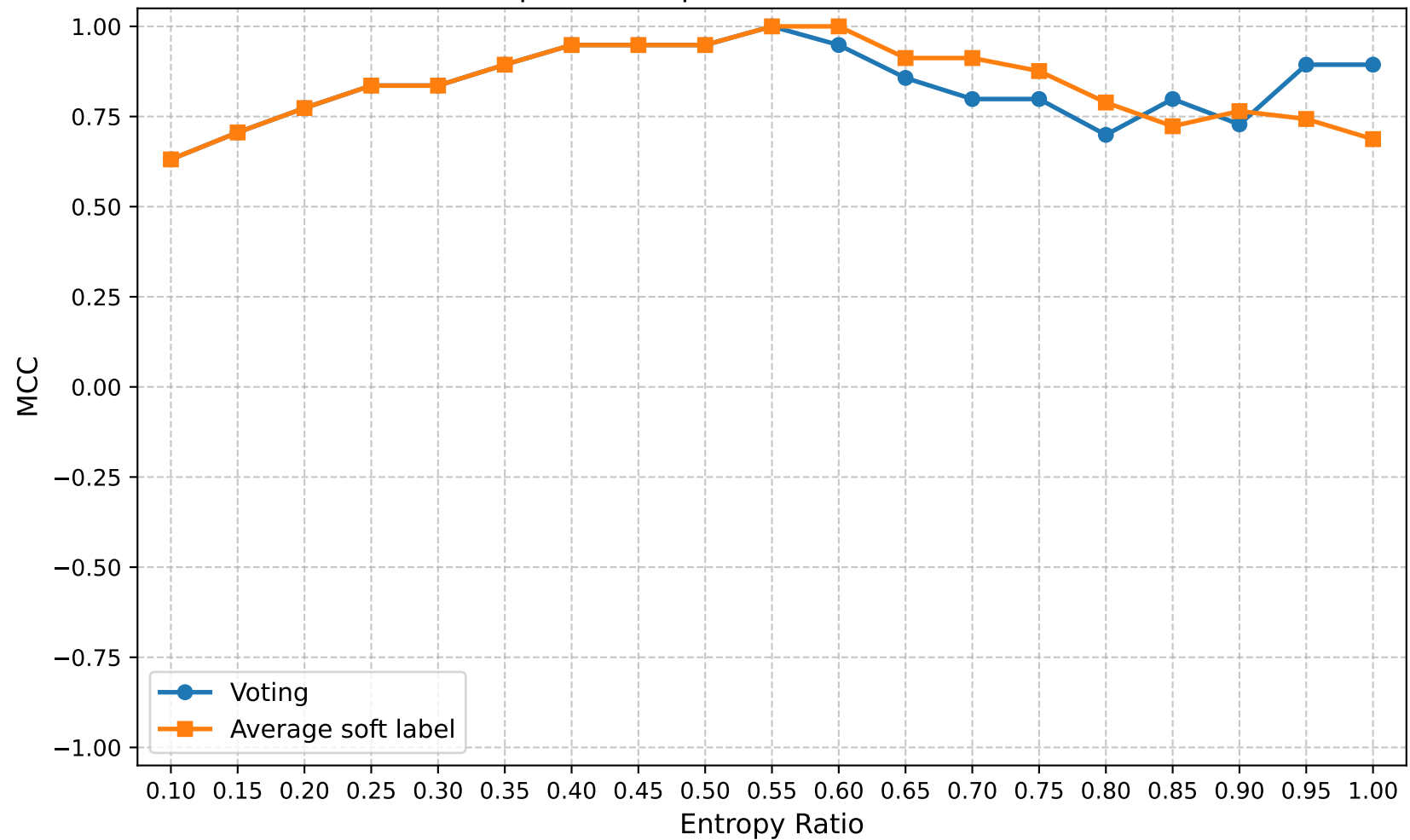
MCC | Round 5 | Confuse Model Ratio 0.70
