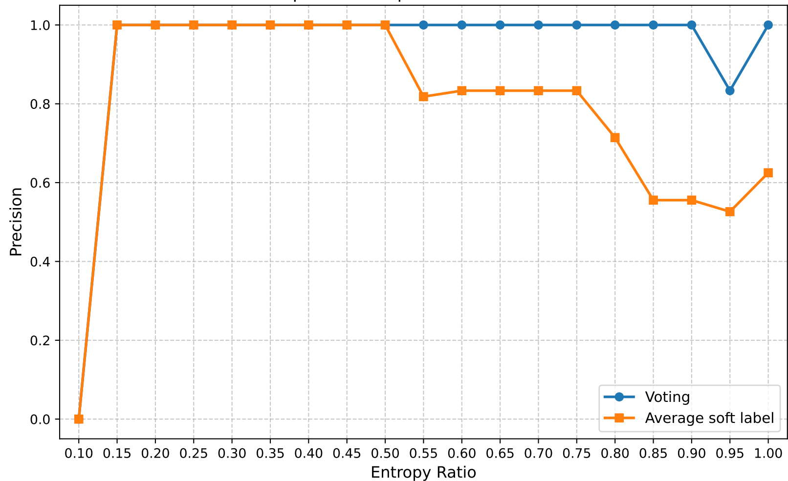
Precision | Round 20 | Confuse Model Ratio 0.50
