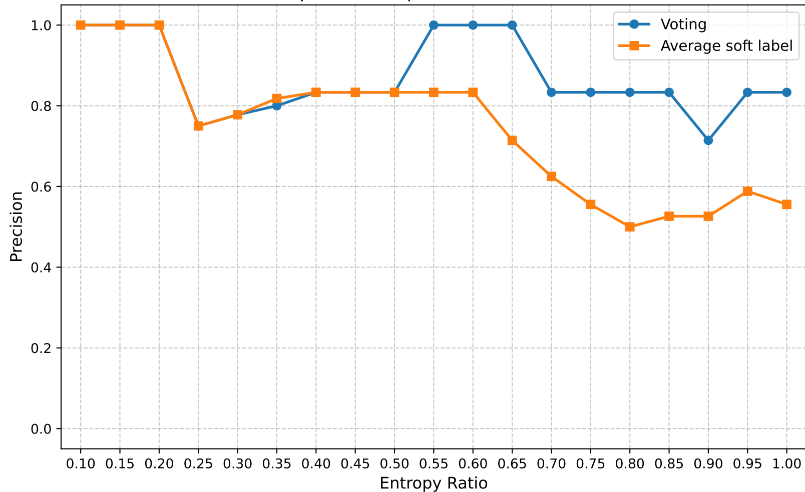
Precision | Round 25 | Confuse Model Ratio 0.70
