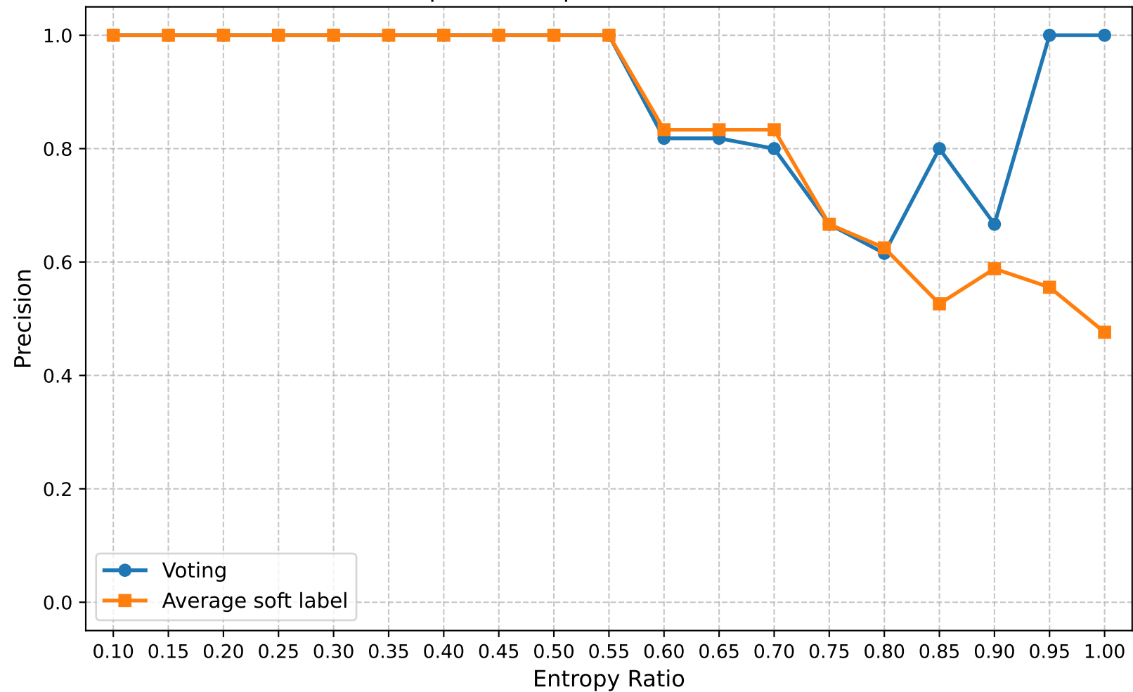
Precision | Round 5 | Confuse Model Ratio 0.80
