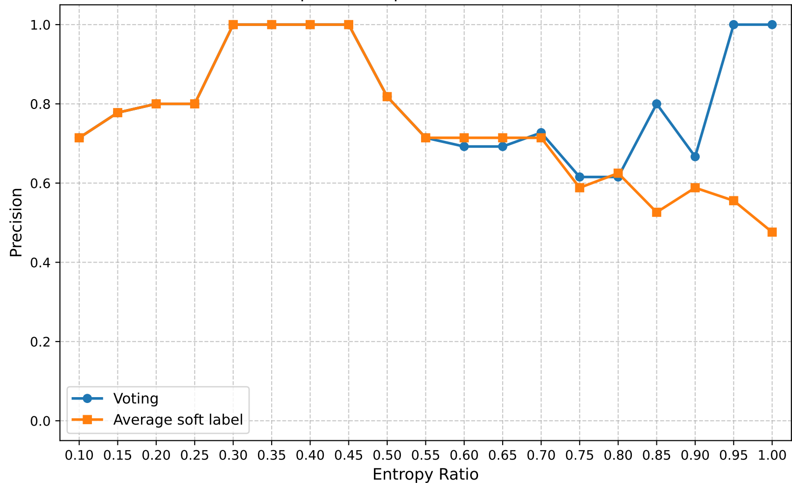
Precision | Round 5 | Confuse Model Ratio 0.90
