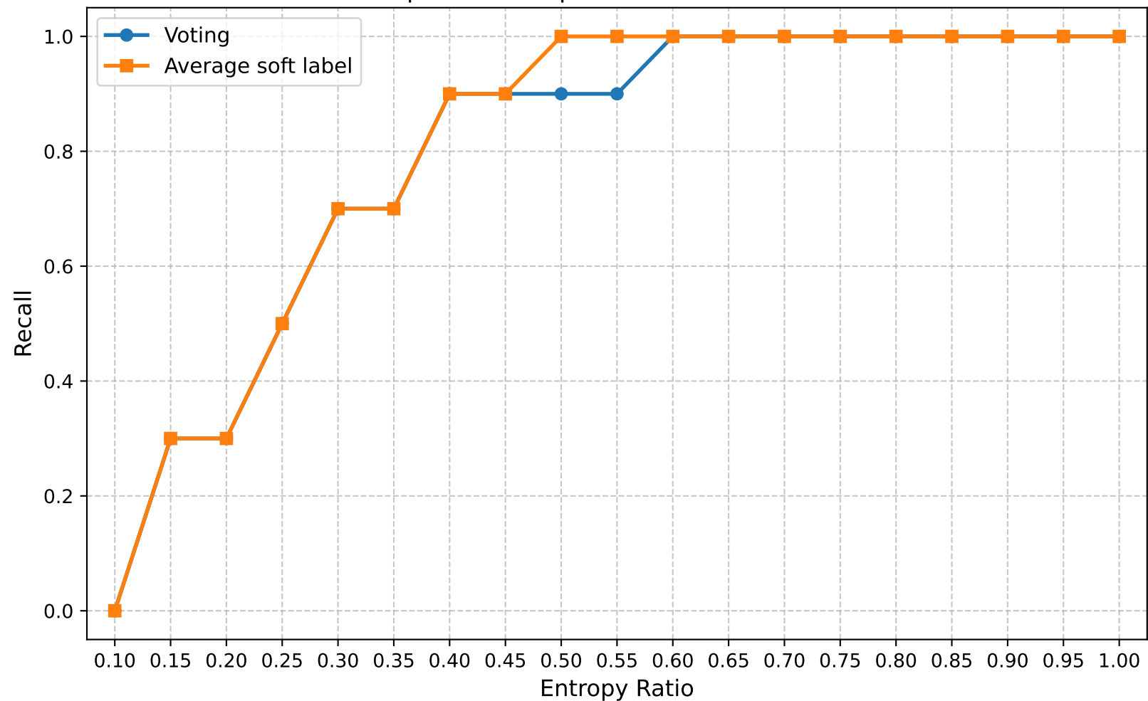
Recall | Round 10 | Confuse Model Ratio 0.60
