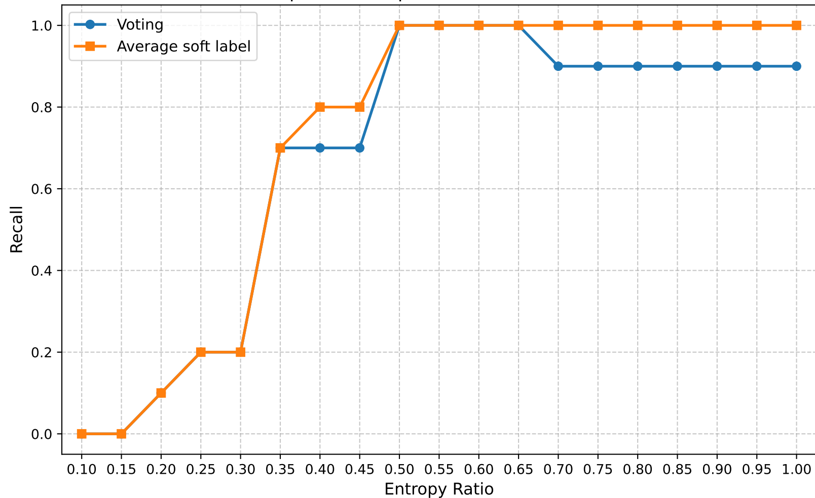
Recall | Round 15 | Confuse Model Ratio 0.40
