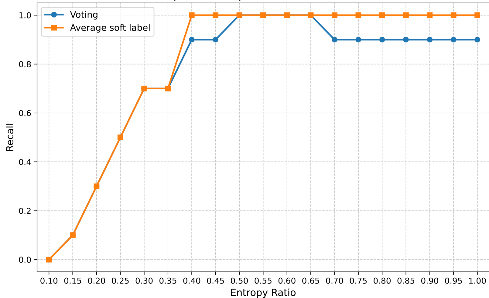
Recall | Round 15 | Confuse Model Ratio 0.60
