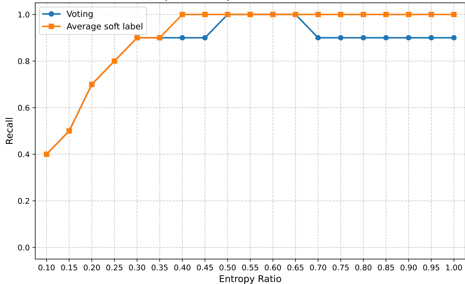
Recall | Round 15 | Confuse Model Ratio 0.90
