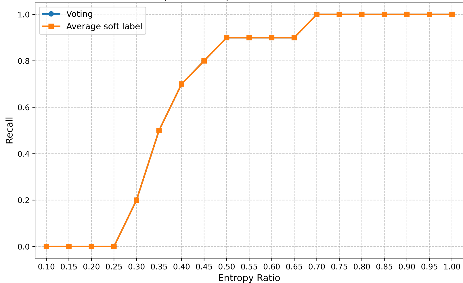
Recall | Round 20 | Confuse Model Ratio 0.30
