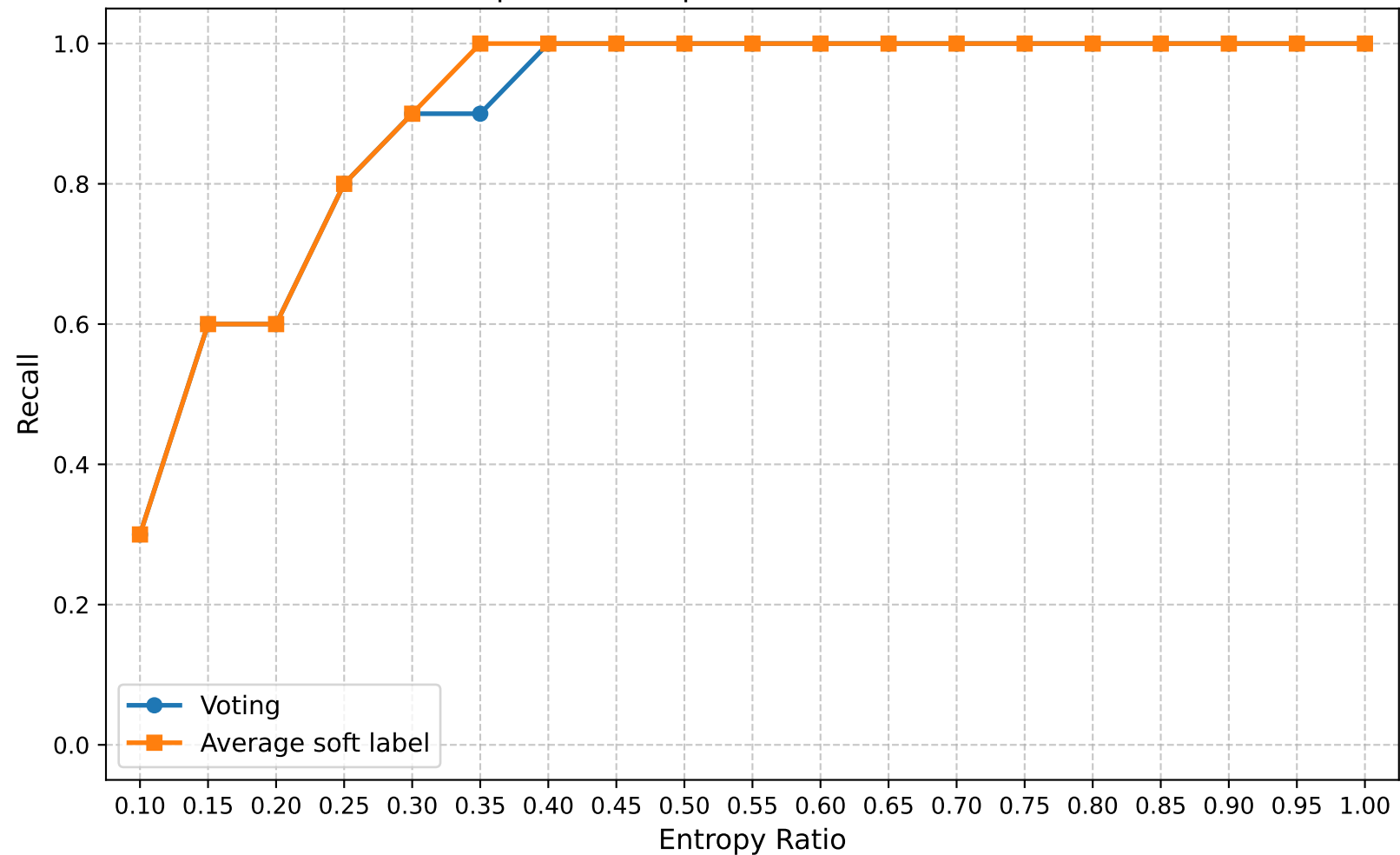
Recall | Round 20 | Confuse Model Ratio 1.00
