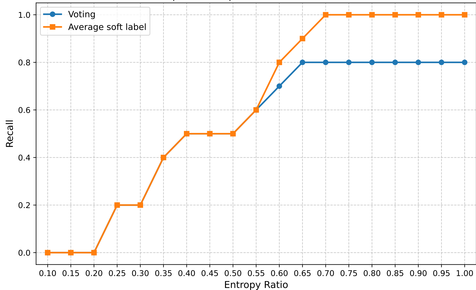
Recall | Round 5 | Confuse Model Ratio 0.10
