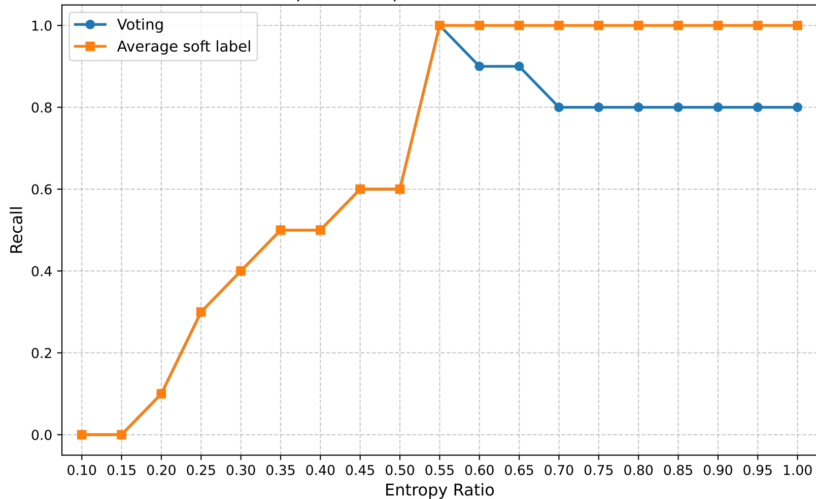
Recall | Round 5 | Confuse Model Ratio 0.20
