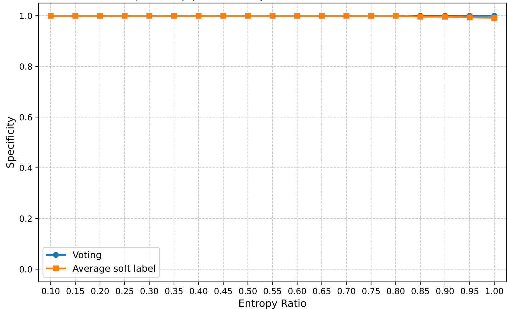
Specificity | Round 15 | Confuse Model Ratio 0.30
