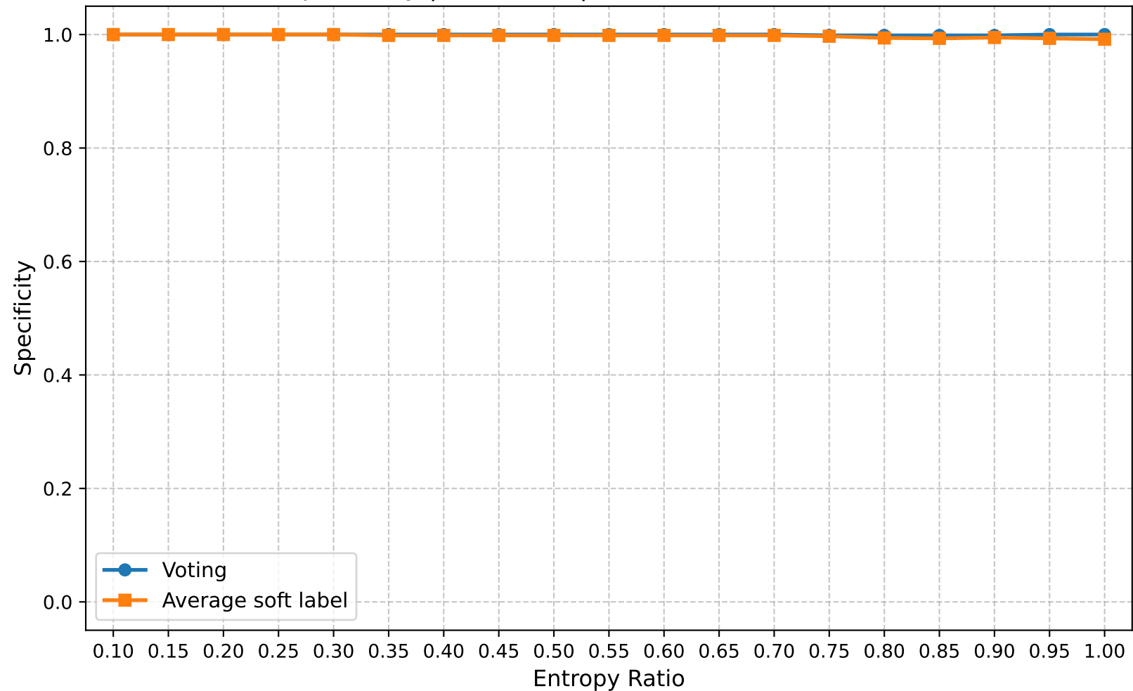
Specificity | Round 15 | Confuse Model Ratio 0.60
